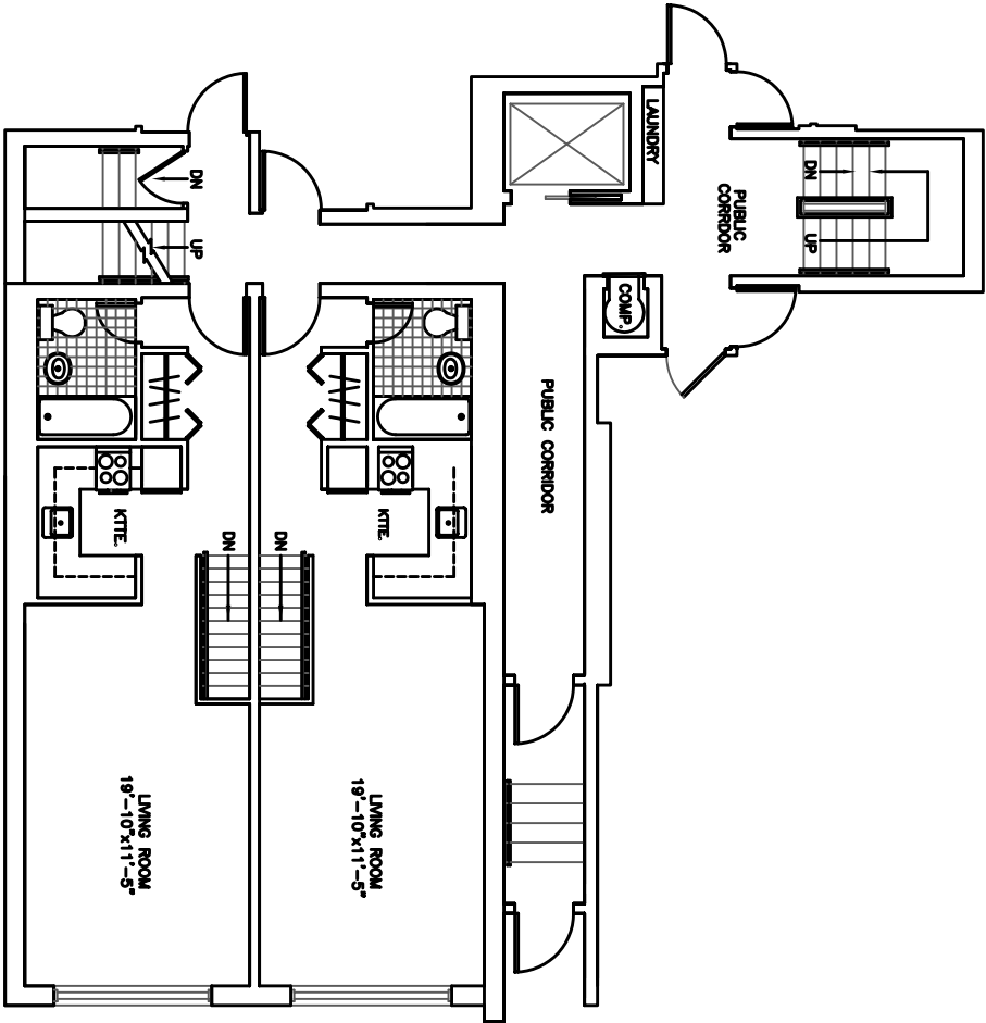
UNIT GH 211-213 E. 73RD ST. 1ST FL. (UPPER LEVEL) 0 1" 2" 6' 12' 24'
