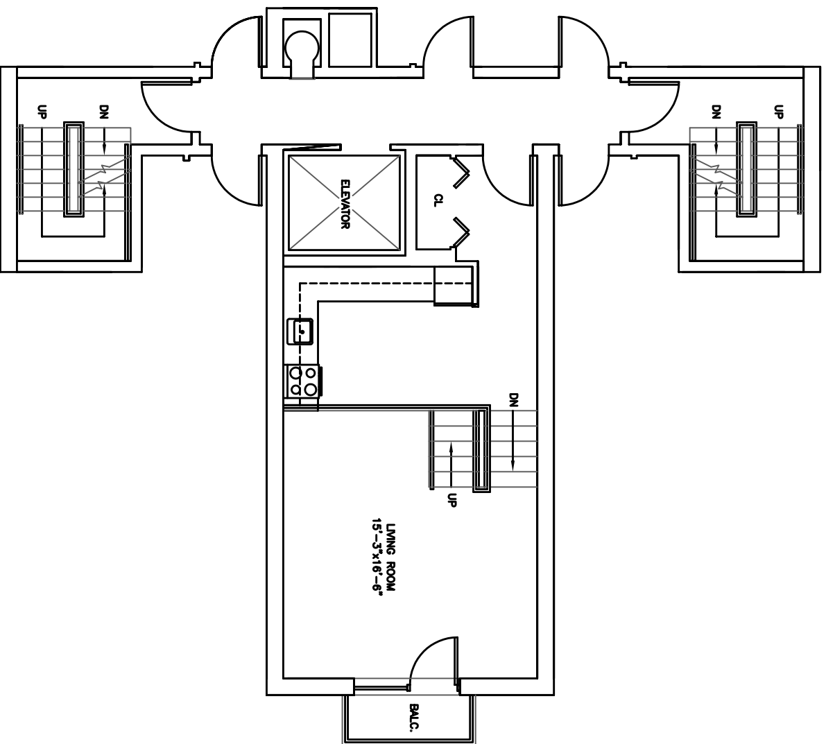
UNIT E 106-107 LEXINGTON AVENUE, 3RD FL. (LOWER LEVEL)
