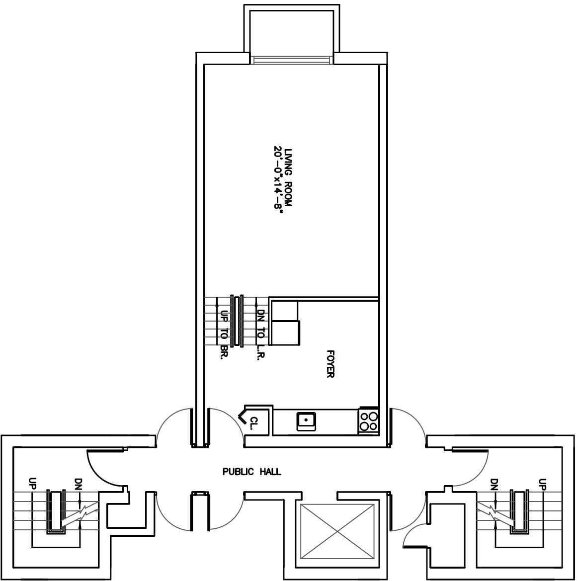
UNIT B 369 EAST 62ND ST. 2ND & 4TH & 6TH FL. (LOWER LEVEL)
